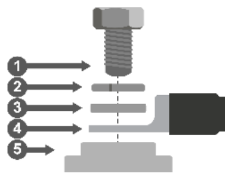
Battery cable connection
