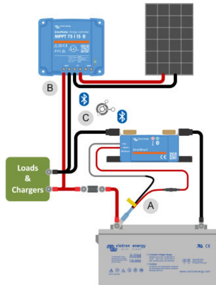
Example of a system containing a battery monitor with a temperature sensor and a solar charger, both using the VE.Smart networking.
