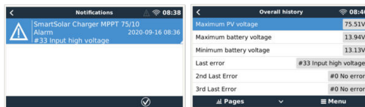
GX device showing alarm notification and historic errors.
