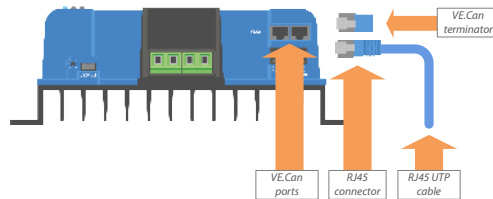
VE.Can port, connector, terminator and cable
