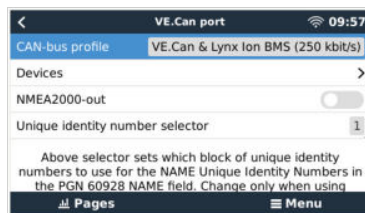
GX screen showing the CAN-bus profile setting
