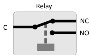
Relay configuration
