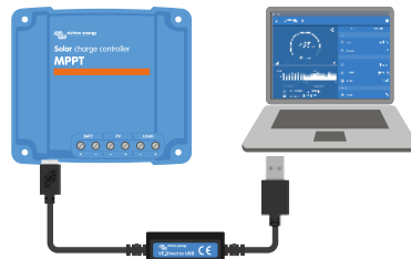
VictronConnect App connection via USB using a VE.Direct USB interface
